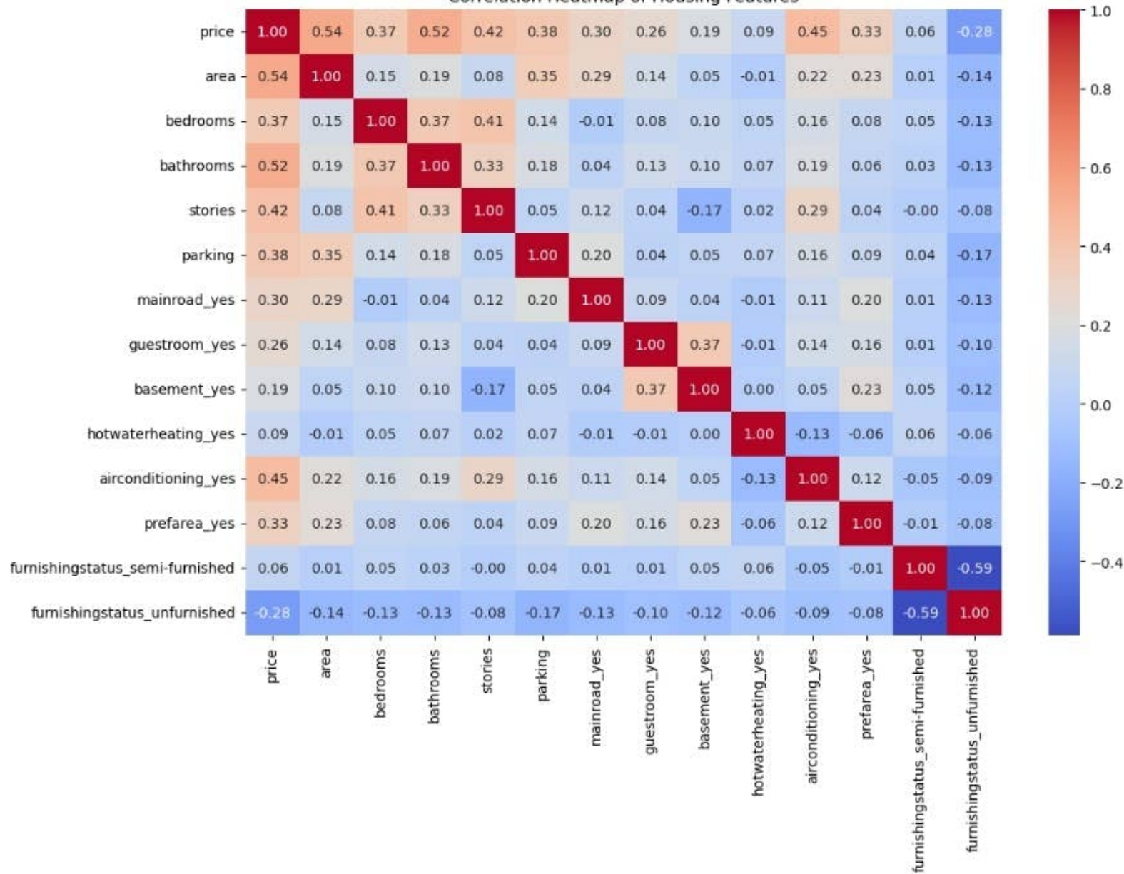
Correlation Heatmap of Housing Features
