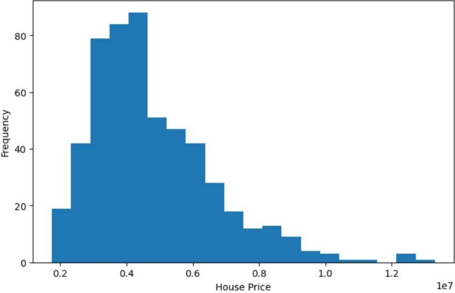
Distribution of House Prices
